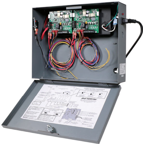
PS124D-10A8 10 AMP / 8 Output 12 and 24 VDC Power supply in metal housing
